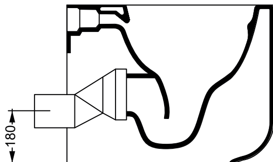
Raccordo eccentrico per connessione a parete. ACS 111PE Offset pan connector to connect wc to the wall line. ACS 111PE
