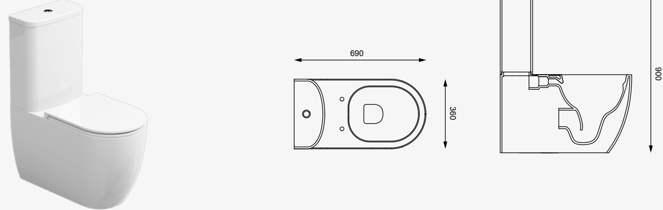
cod. LKMBL / LKCIMBL Vaso monoblocco Like con cassetta WC monoblock Like with cistern
