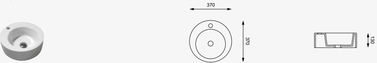
cod. RILAV Lavabo Ring cm. 37 Ring Washbasin cm. 37
