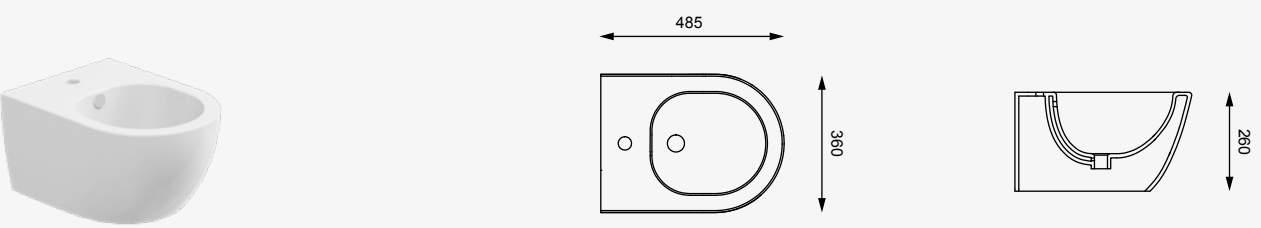
cod. LKBISOXXS Bidet Like sospeso ridotto Bidet Like wall-hung reduced
