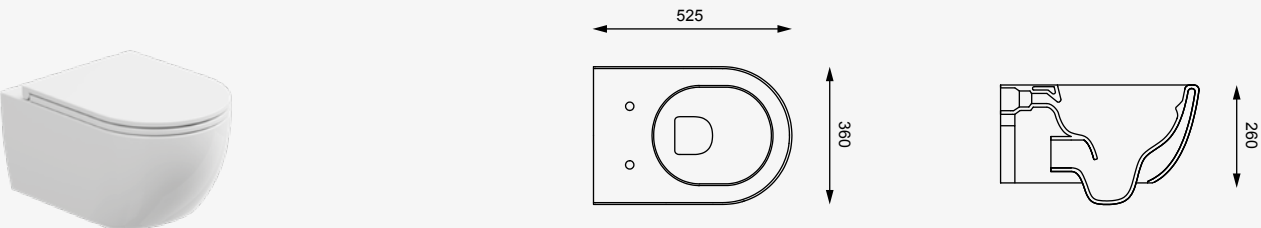
cod. LKWCSO Vaso Like sospeso WC Like wall-hung
