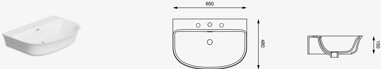
cod. FLLAVBW65 Lavabo a parete Flut da appoggio o sospeso cm. 65 Back to wall washbasin, coutertop or wall-hung Flut cm. 65
