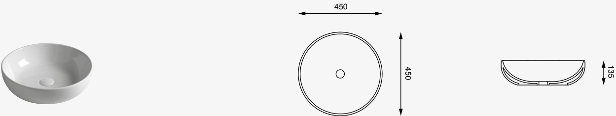
cod. EALAVRO45 Lavabo Easy Tondo cm. 45 Easy Washbasin Round cm. 45
