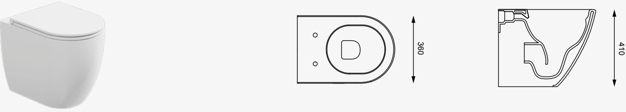
cod. LKBI0155 Bidet Like a terra Bidet Like back to wall
