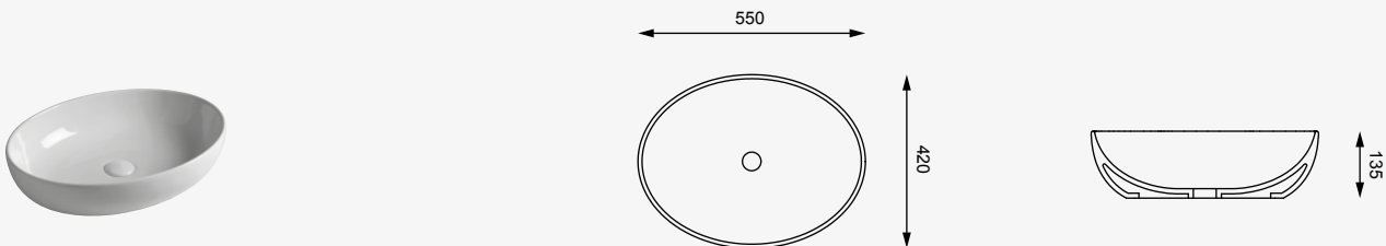
cod. EALAVOV55 Lavabo Easy Ovale cm. 55 Easy Washbasin Oval cm. 55
