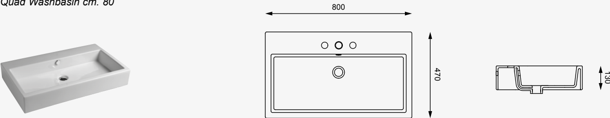
cod. QULAV80 Lavabo Quad cm. 80 Quad Washbasin cm. 80
