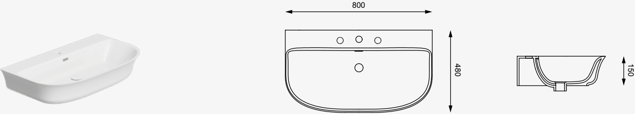
cod. FLLAVBW80 Lavabo a parete Flut da appoggio o sospeso cm. 80 Back to wall washbasin, coutertop or wall-hung Flut cm. 80
