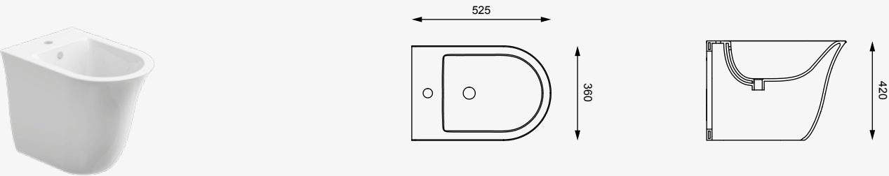
cod. FLBI01 Bidet a terra Flut Bidet back to wall Flut
