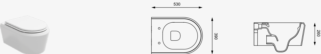
cod. CRWCSO Vaso Cruise sospeso WC Cruise wall-hung
