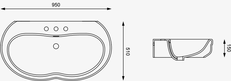
cod. TILAV95 Lavabo Time a parete cm. 95 da appoggio, sospeso o su colonna, Countertop, wall-hung back to wall or on pedestal washbasin Time cm. 95 with pedestal
